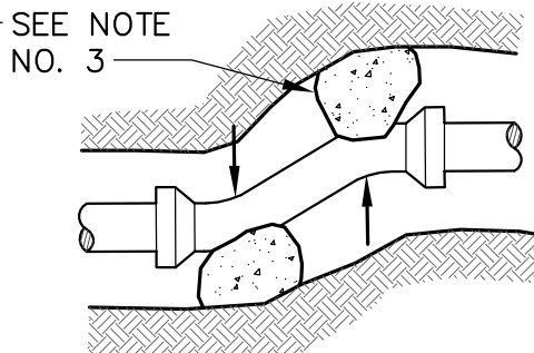
OFFSET
