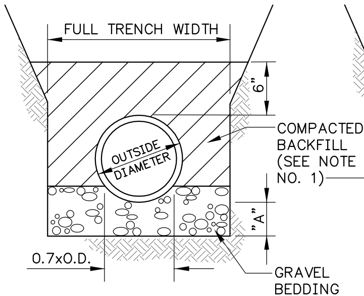
CLASS C SHALLOW GRAVEL BEDDING
