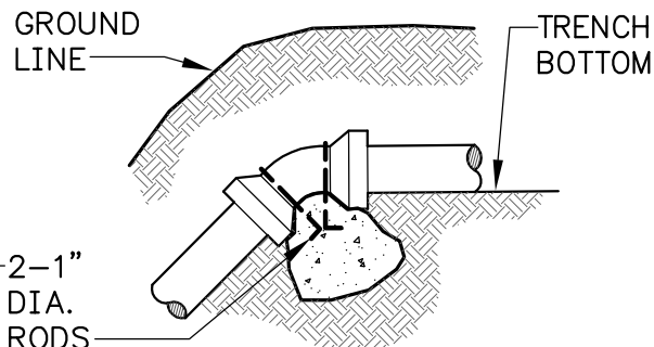
VERTICAL BEND
