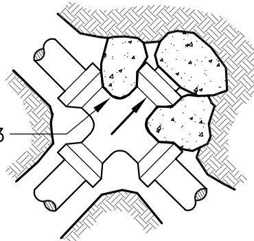
PLUGGED CROSS
